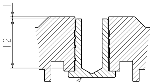
M6 INSERT NUT A-A 2:1 4 THREADS DETAILS
